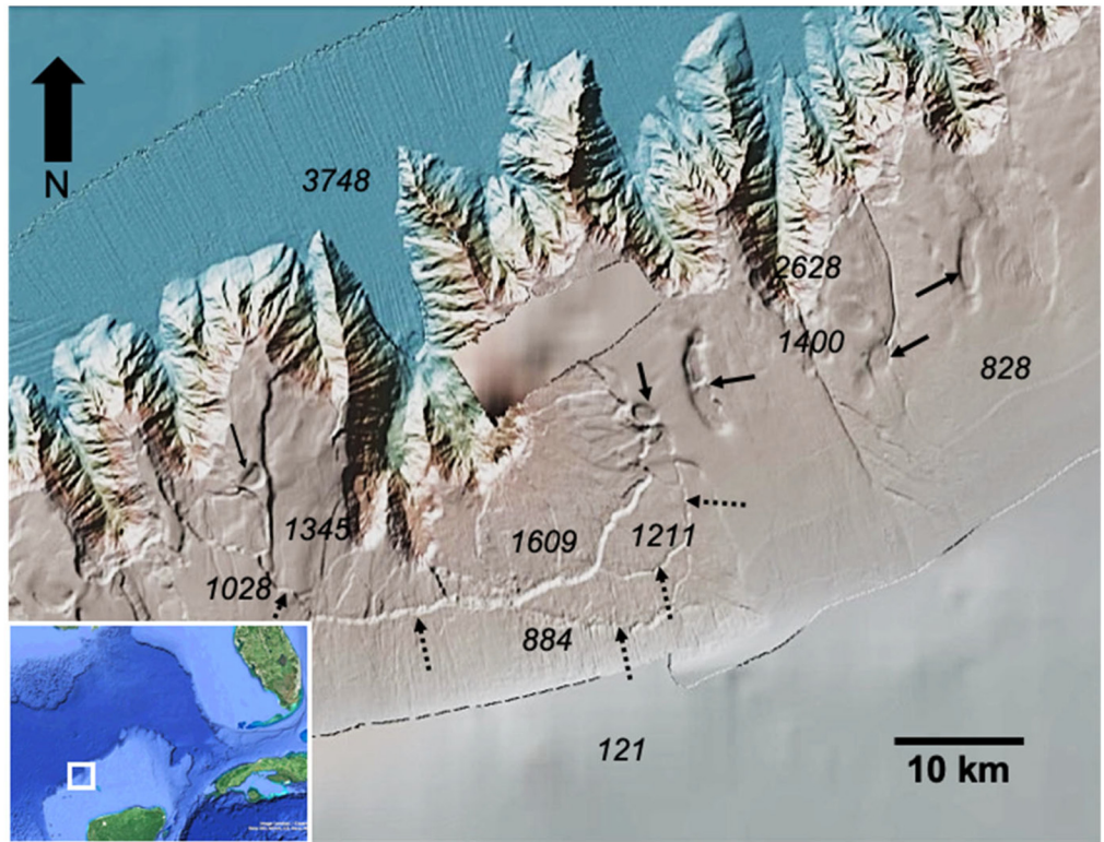
Figure 8. A portion of the Yucatán Escarpment. Location shown by white box in the inset. Italicized numbers are water depths in meters. Solid black arrows indicate sinkholes. Dashed black arrows indicate possible wave cut benches. Timing of incision is admittedly poorly constrained, but the smooth canyon floor that presumably buries the removed talus argues against Pleistocene slope failure. Image from Polar Explorer web app. Inset image from Google Earth.
