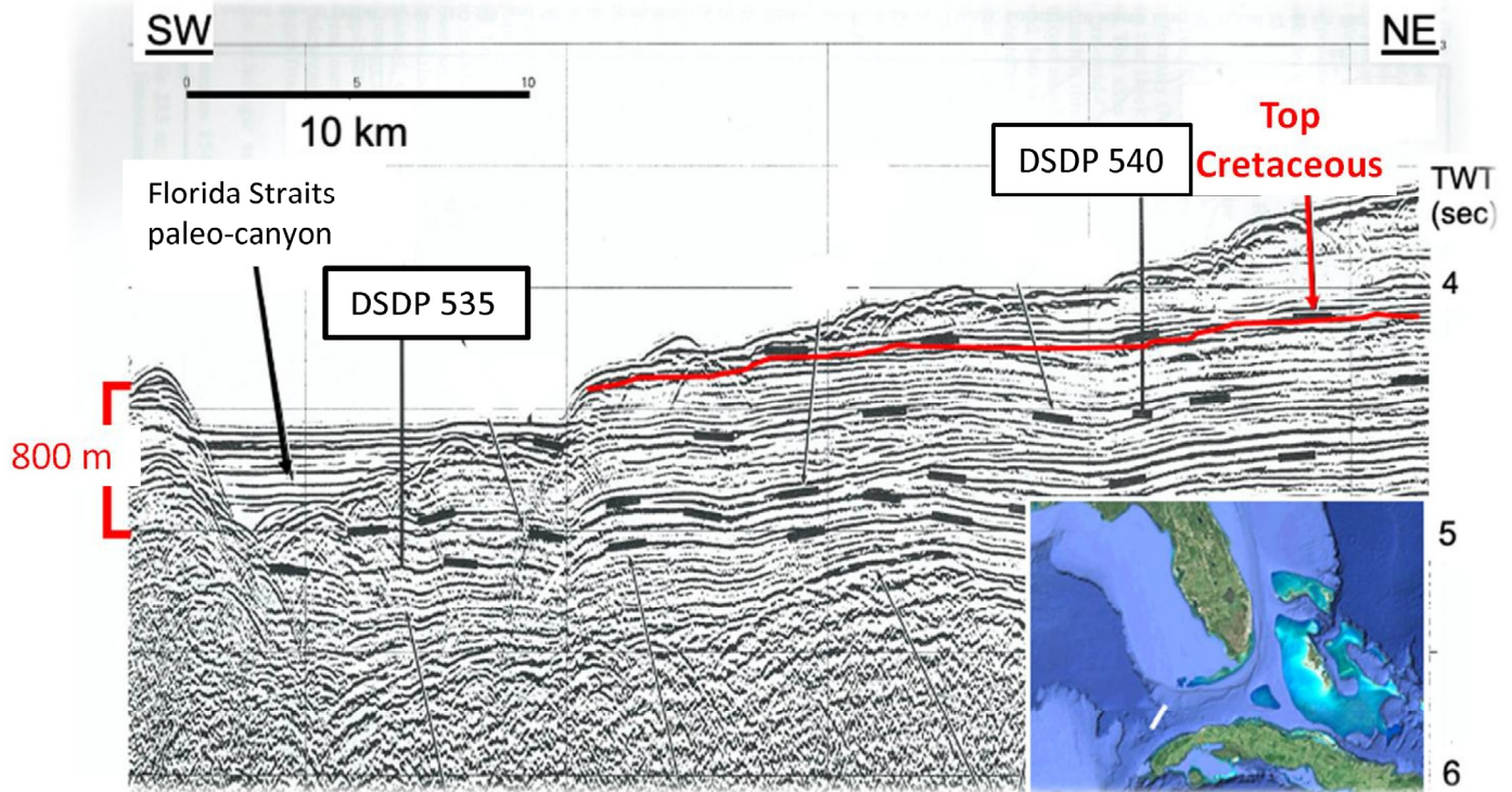
Figure 9. Seismic line across the western end of the Florida Straits paleo-canyon (modified after Buffler et al., 1984). Location shown by the white line in the inset. Note 800-meter relief from thalweg to top of canyon wall. DSDP 535 drilled Pleistocene sediments overlying mid-Cretaceous deepwater carbonates in the canyon but the oldest canyon fill sediments were not drilled.
