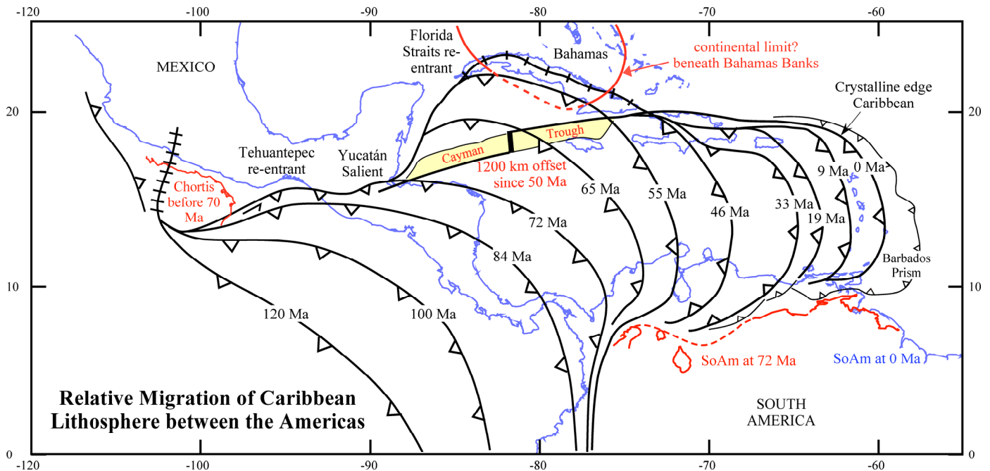
Figure 2. “Sweep of the Antillean Arc of the Caribbean” between the Americas, modified after Pindell and Barrett (1990) , Pindell and Kennan (2001, 2009) , and Pindell et al. (2005, 2006) . Relative motion is actually driven by westward drift of the Americas over the mantle; Caribbean has been stationary in the mantle reference frame for most of the Cenozoic. Cayman Trough began to open in the Eocene, thereby stranding Cuba and the Yucatán Basin with the North American Plate and allowing the rest of the Caribbean to move relatively east without them.
